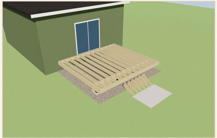
Frame only — joists, rims, beams, ledger
