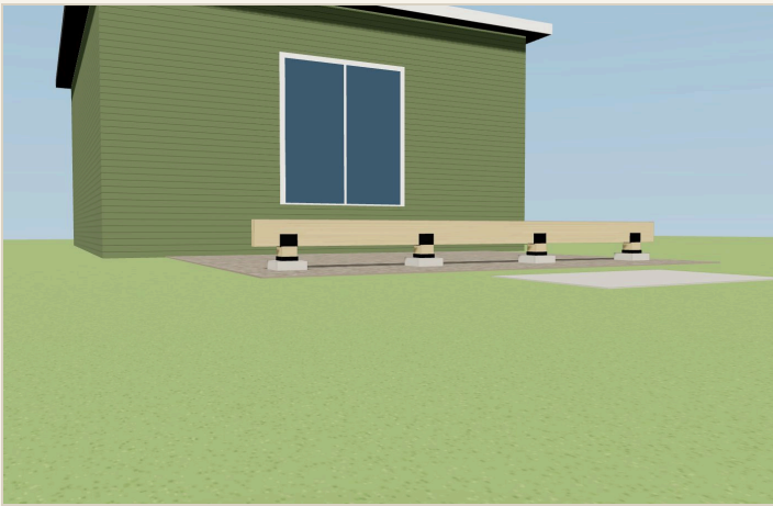
Posts and beams on the footings
